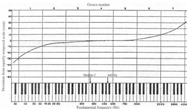
グラフ1 Railsback stretch in piano tuning 注1
